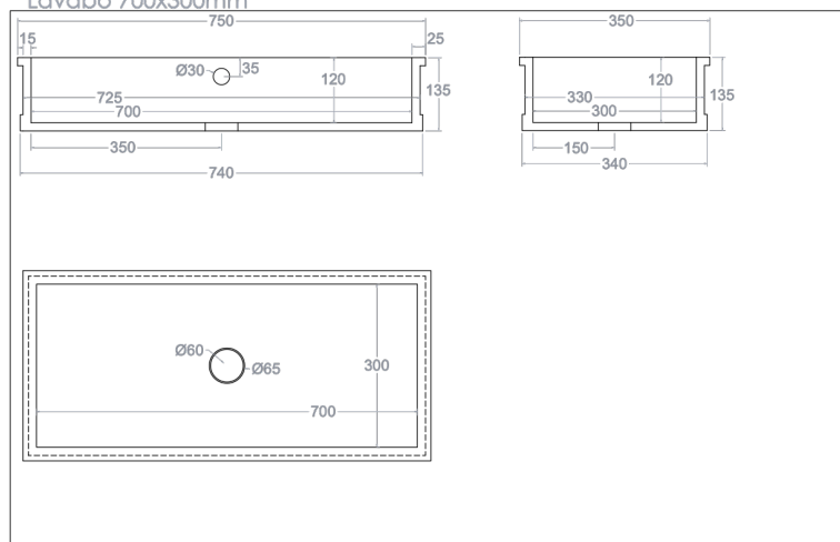
Lavabo 700x300mm
